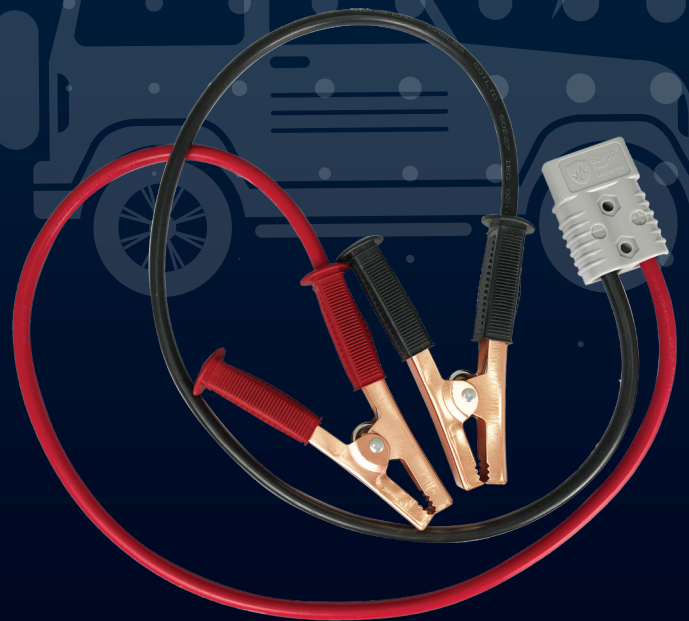
Optional 175A jump starter cable (Part No. HKPBATTWIR)
